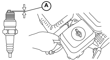
Figure 4-8. Spark Plug
